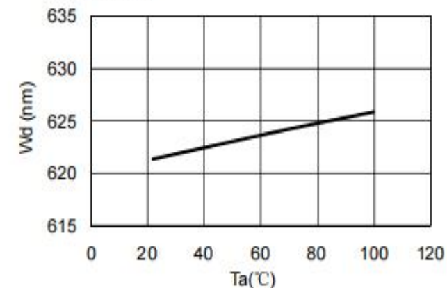
Fig.5-Dominant Wavelength (@20mA) vs. Ambient Temperature
